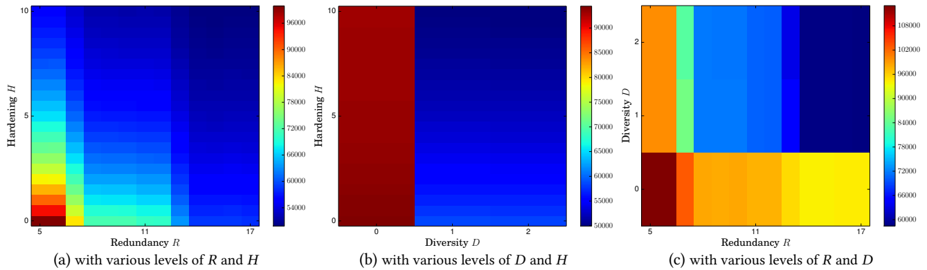
Figure 2: Expected impact of cyber-physical attacks with various levels of redundancy R , diversity D , and hardening H .
